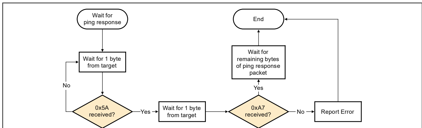
Figure 37. Host Reads Ping Packet from Target via LPUART
