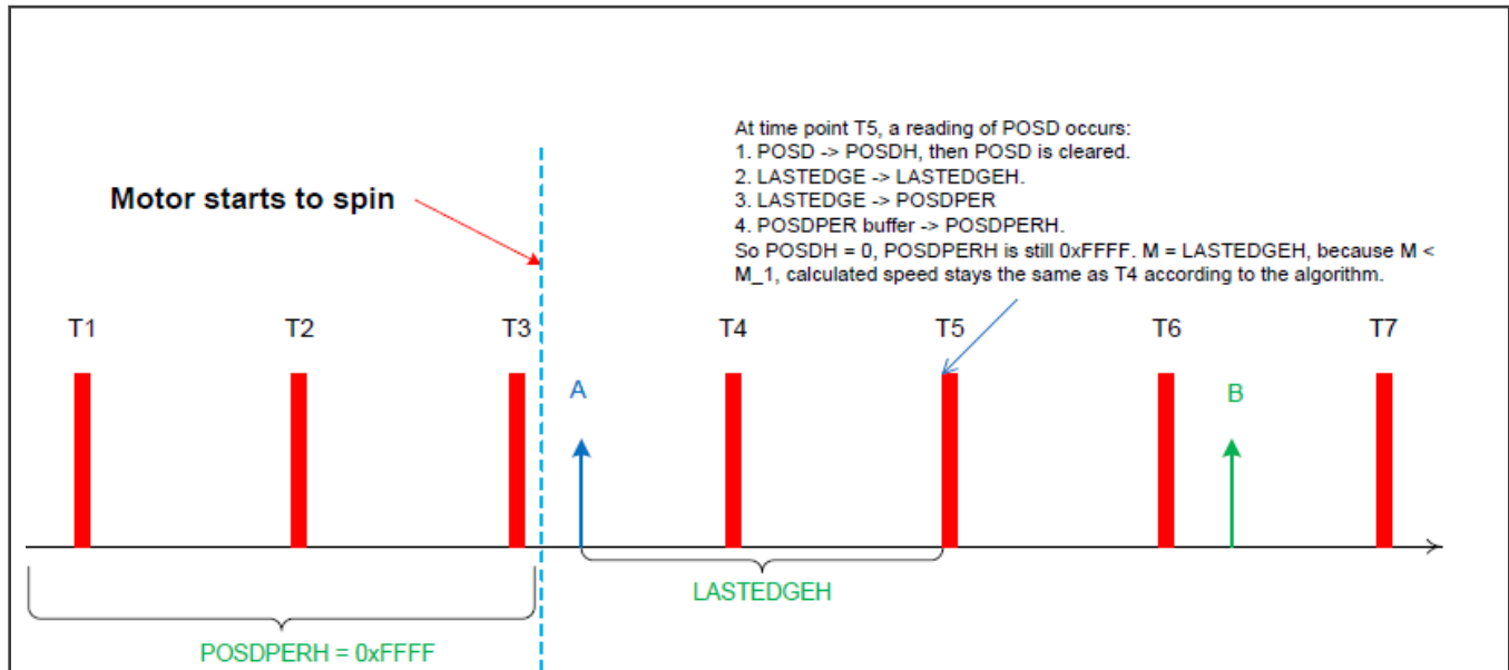
Figure 138. Speed measurement at time point T5
