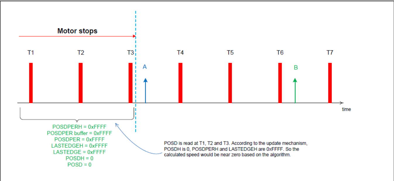
Figure 136. Speed measurement at time point T1~T3
