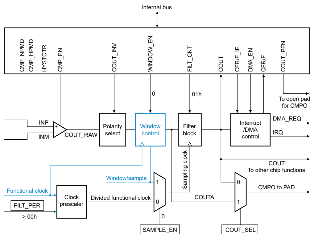
Figure 175. Sampled, Non-Filtered (#3B): sampling interval internally derived
