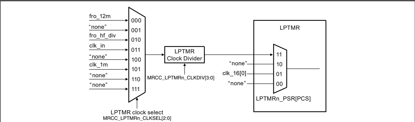
Figure 54. LPTMR clock
