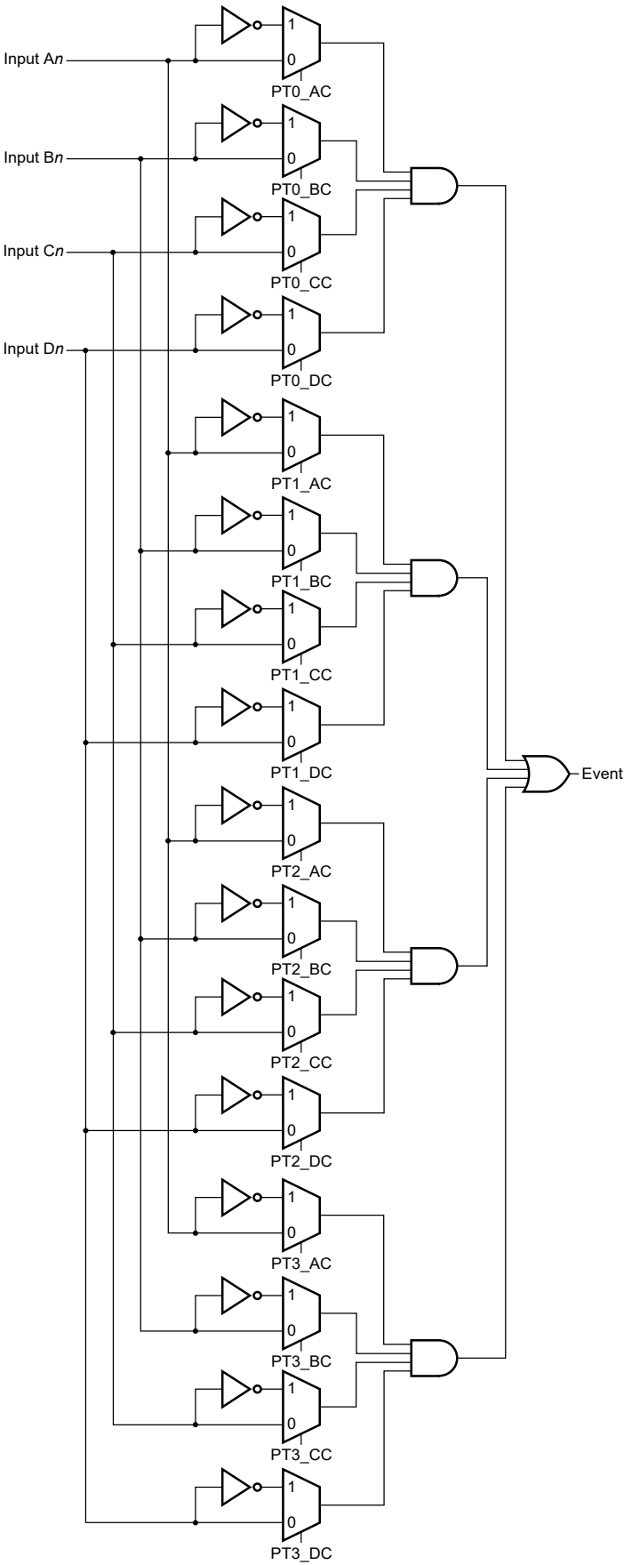
Figure 25. Block diagram MCX A153, A152,A143, A142, A133, A132 Reference Manual, Rev. 5, 08/2024
