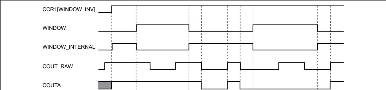
Figure 184. Windowed mode timing diagram with window signal inverted
