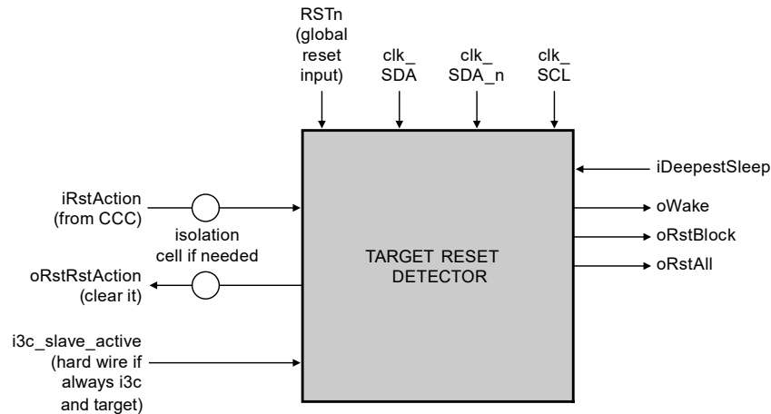
Figure 166. Showing reset detector connections — not all used in many systems
