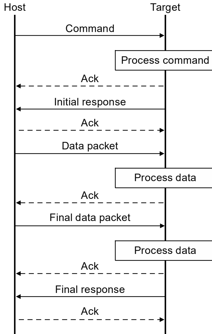
Figure 34. Command with incoming data phase
