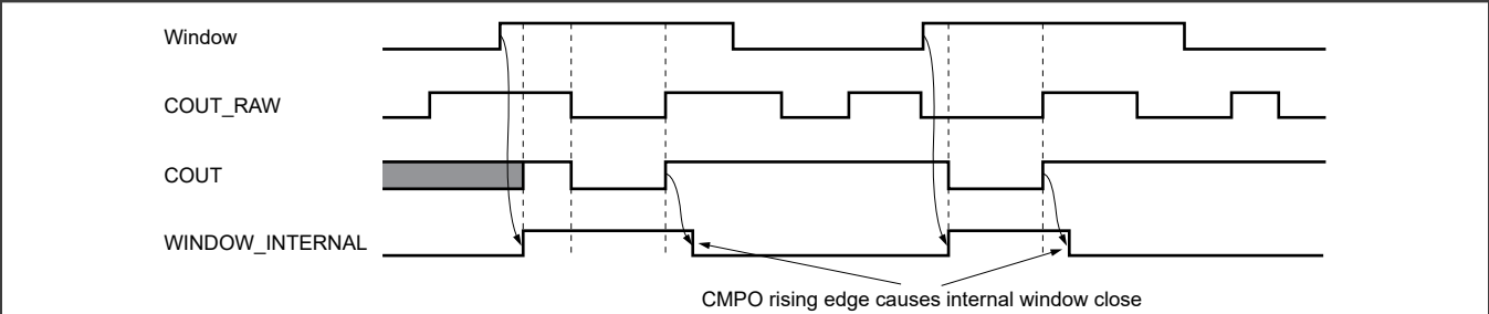
Figure 183. Windowed mode timing diagram with COUT rising edge close window
