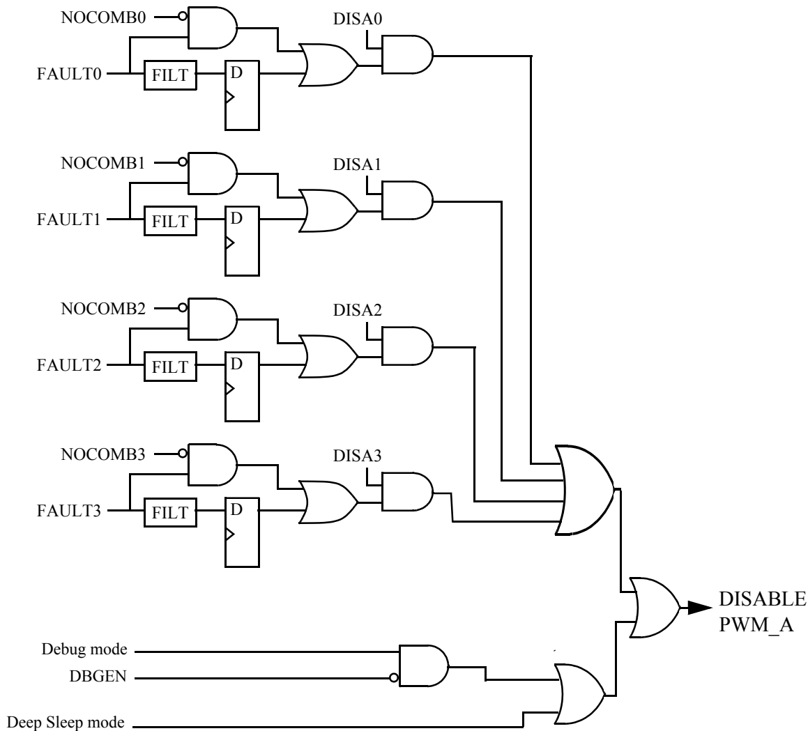
Figure 111. Fault decoder for PWM_A
