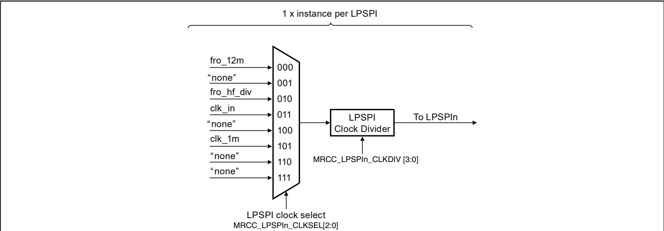
Figure 53. LPSPI clock
