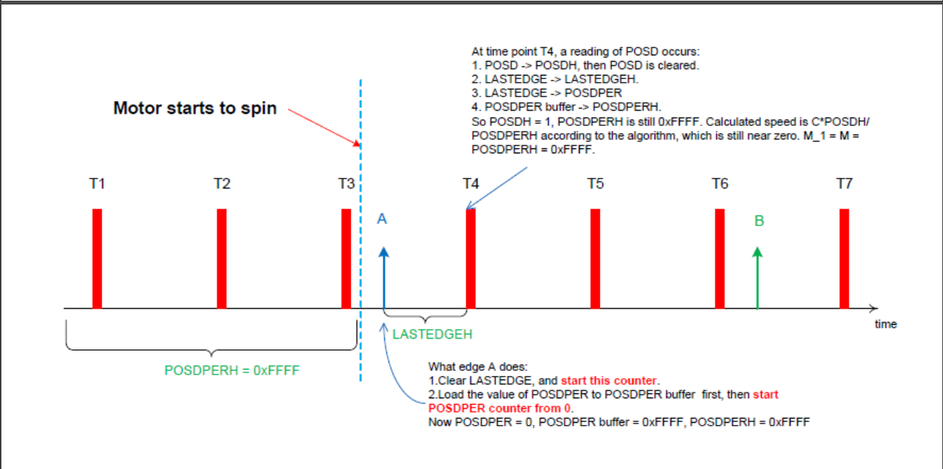
Figure 137. Speed measurement at time point T4
