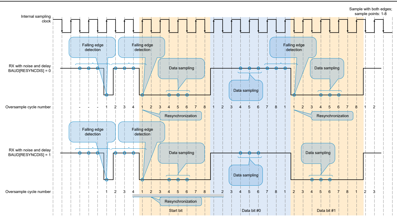
Figure 159. LPUART resynchronization diagram
