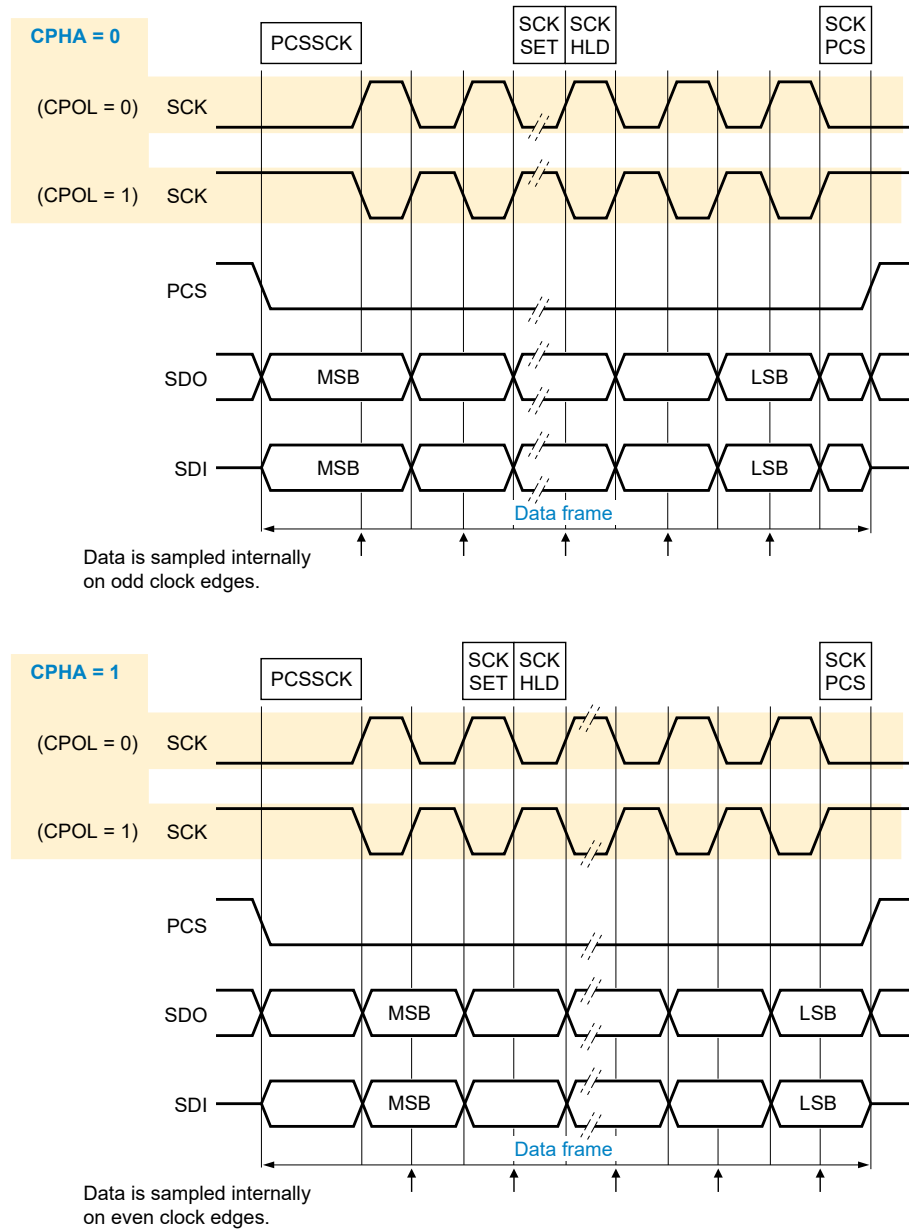
Figure 161. Clock phase (TCR[CPHA]) timing diagram example
