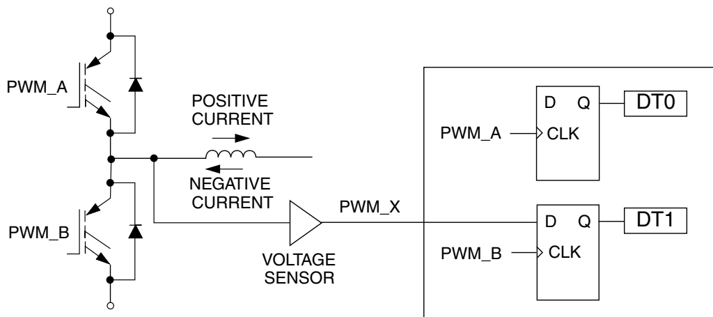
Figure 106. Current-status sense scheme for deadtime correction
