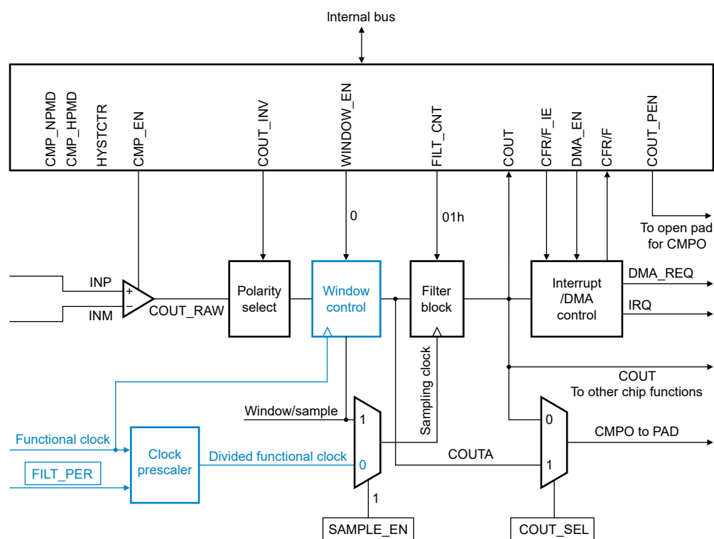
Figure 174. Sampled, non-filtered (#3A): sampling point externally driven
