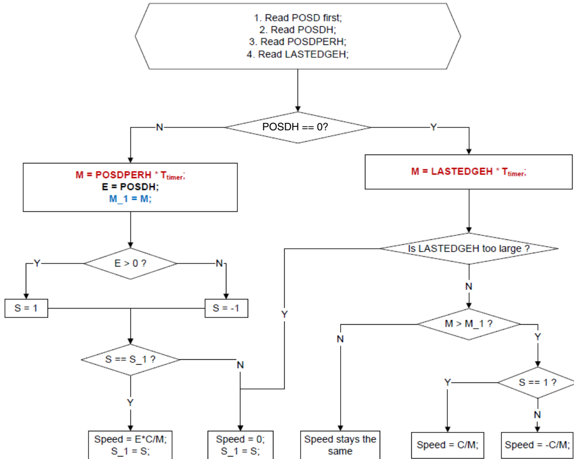
Figure 135. Flowchart of speed calculation with method
