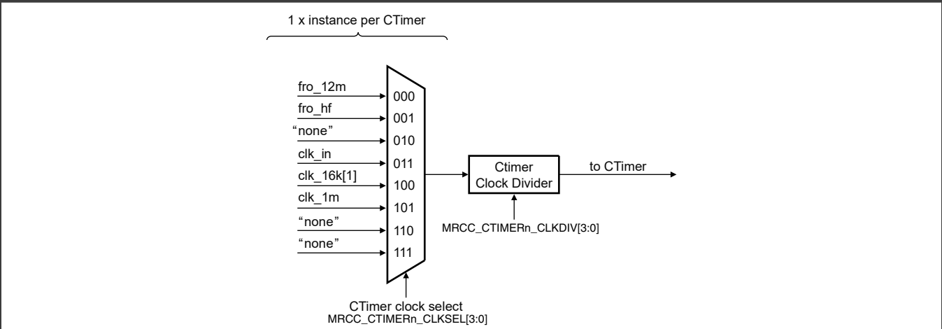
Figure 55. CTimer clock
