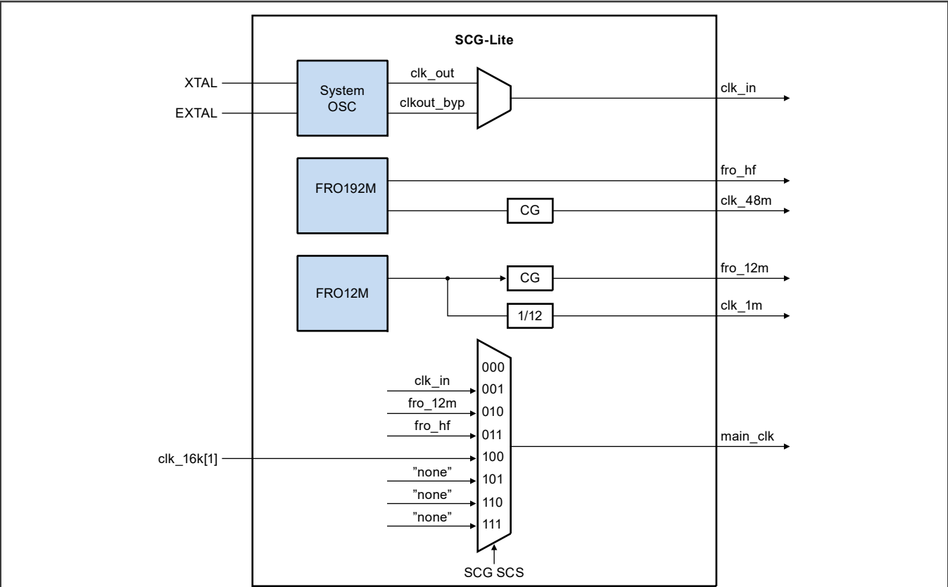
Figure 40. SCG clock
